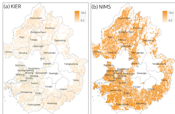
Fig. 1. Market potential of PV: KIER vs. NIMS ( \text{MWh/year/100 m}^2 )
